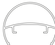
Main courante ronde Ref. 180033 Section 60 x 48mm
